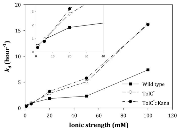
Figure 2. Average deposition rate coefficients ( k_d ) for the three E. coli strains under ionic strength conditions of 1, 5, 20, 50, and 100 mM. The error bars, which represent the standard deviations, are smaller than the symbols.
