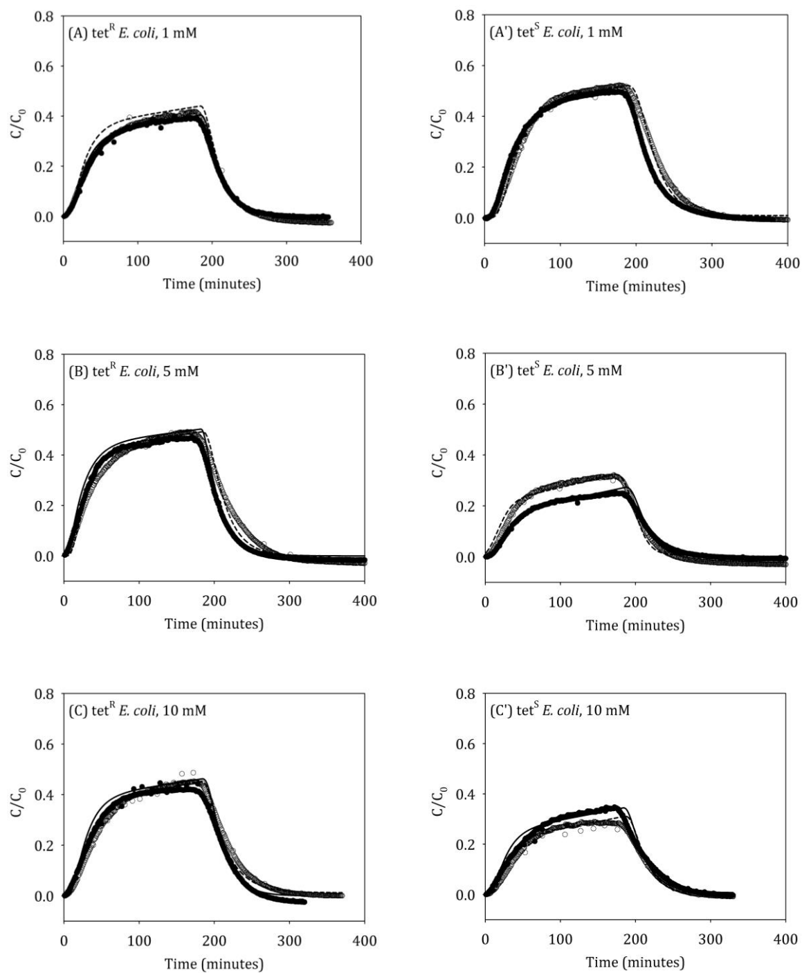
Figure 7. Breakthrough concentrations of the \text{tet}^R (A-C) and \text{tet}^S (A'-C') E. coli strains under ~25% of soil moisture content. Symbols represent experimental observations and lines represent model simulation results.
